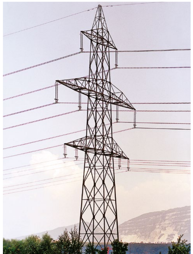
First Suspension/Tension Insulators for 420 kV in 1990
