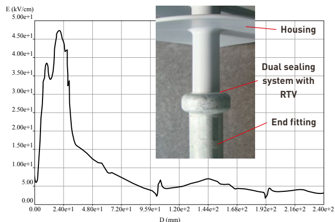
Fig. 25: Sealing by casting with E-field simulation
