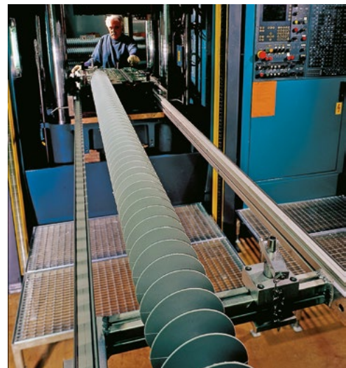
Fig. 20: Multiple high pressure injection moulding
