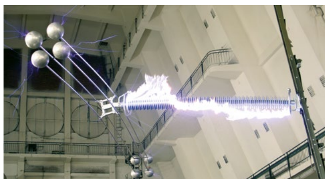
Fig. 30: HV-testing as special demand
