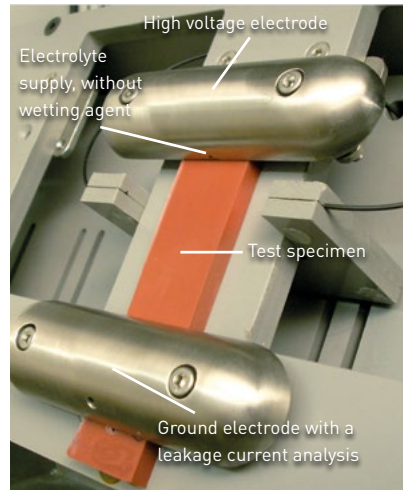
Fig. 10.3: Set-up of the Dynamic Drop Test
