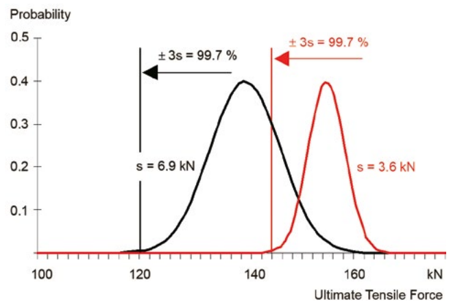
Fig. 18: Improvement by optimized crimp parameters
