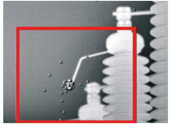
Fig. 38: Corona activity can be measured in daylight
