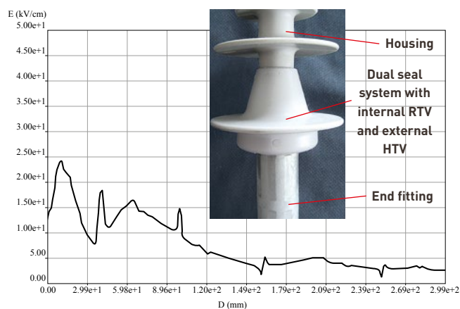
Fig. 27: Sealing by corona shed with E-field simulation
