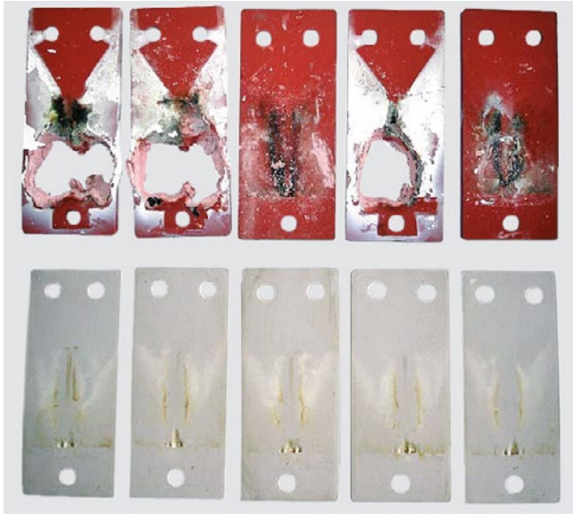
Fig. 9: Erosion resistance of inappropriate filled (top array) and well-balanced (bottom array) Silicone Rubber
