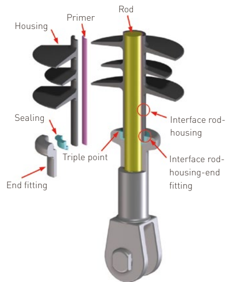
Fig. 1: Parts of a composite insulator
