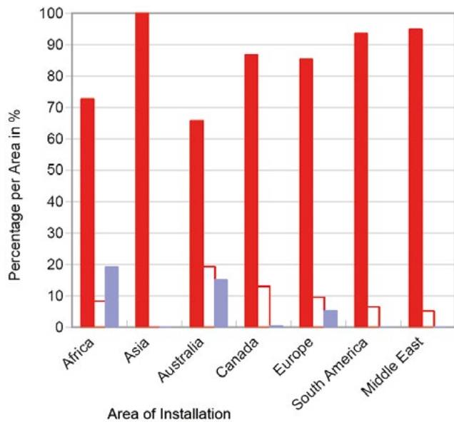
Fig. 6: Use of housing material for composite insulators > 100 kV
