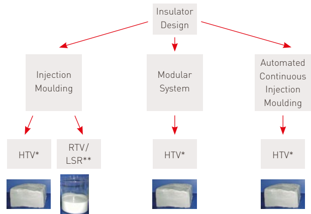
* using high pressure injection moulding ** using low pressure injection moulding Fig. 19: Silicone Rubber processing used at PFISTERER SEFAG
